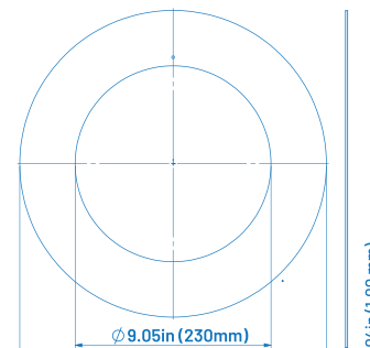
DT GR 10R W - 10" Round Goof Ring
